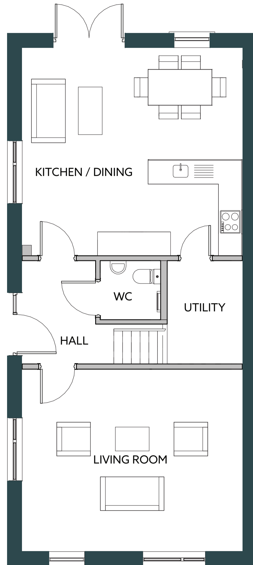
Ground Floor
