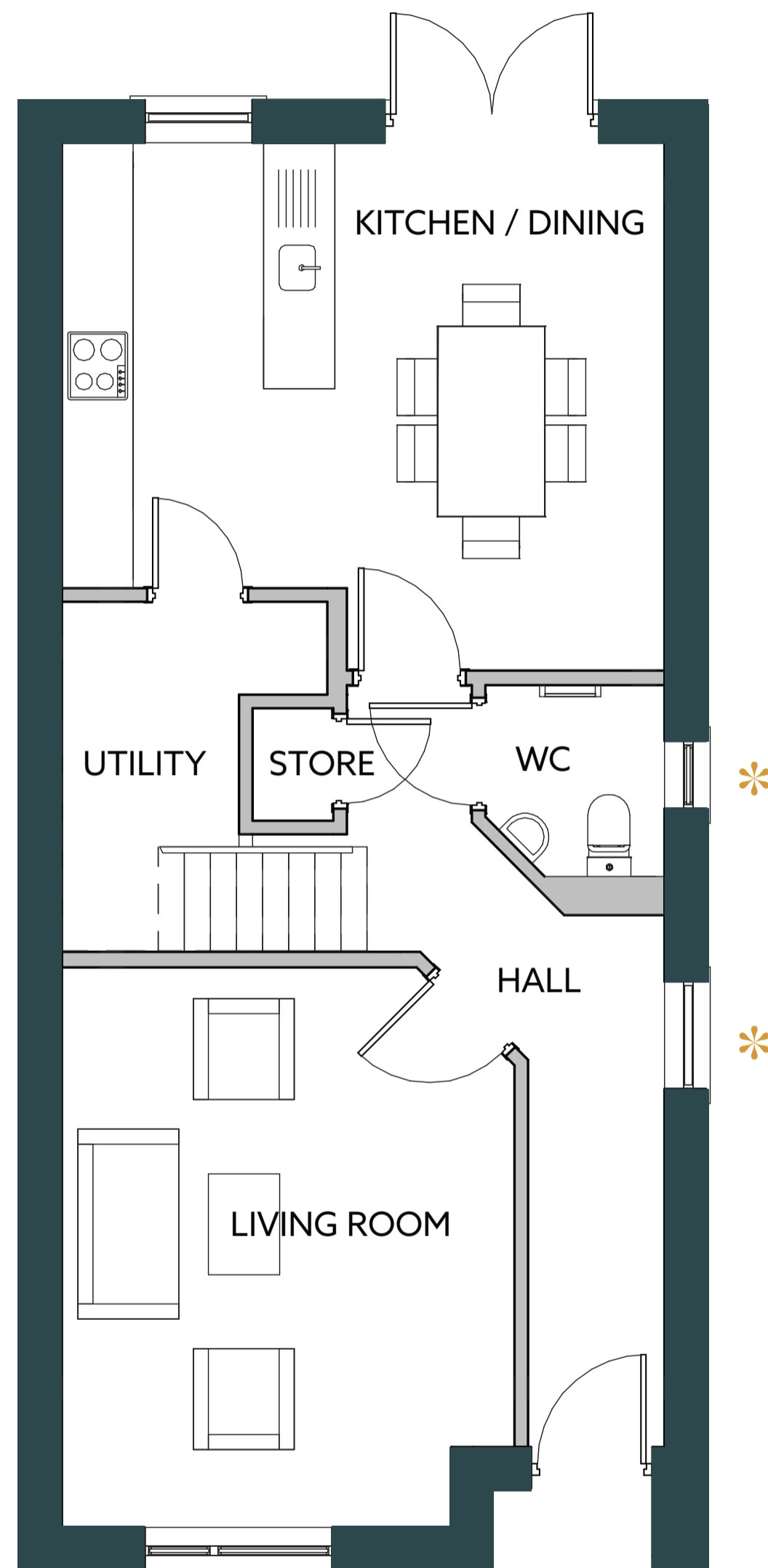
Ground Floor
